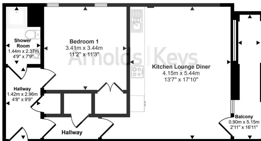
Floorplan
